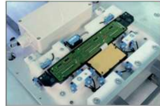
Detecting whether the workpiece is placed in the fixture
